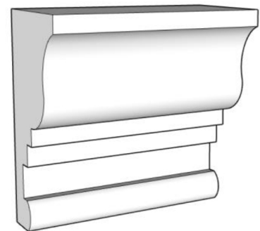
CR150 A B 12-1/4" 5-7/8"
