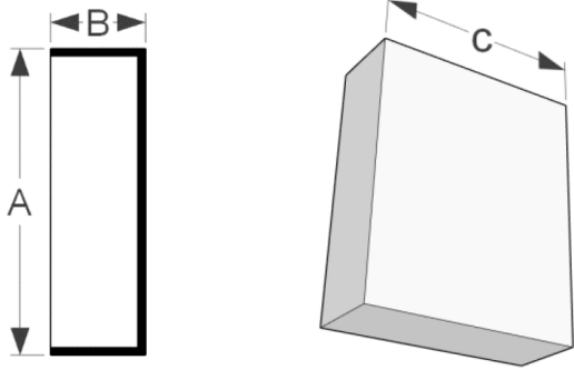
Flat Dentils from Flat Stock "B" Thickness ranges from 1"-3" "C" measurement varies
