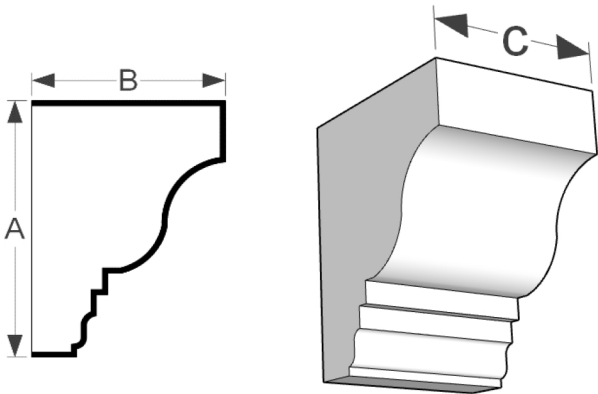
A B C DB130 6" 4-3/4" Varies
